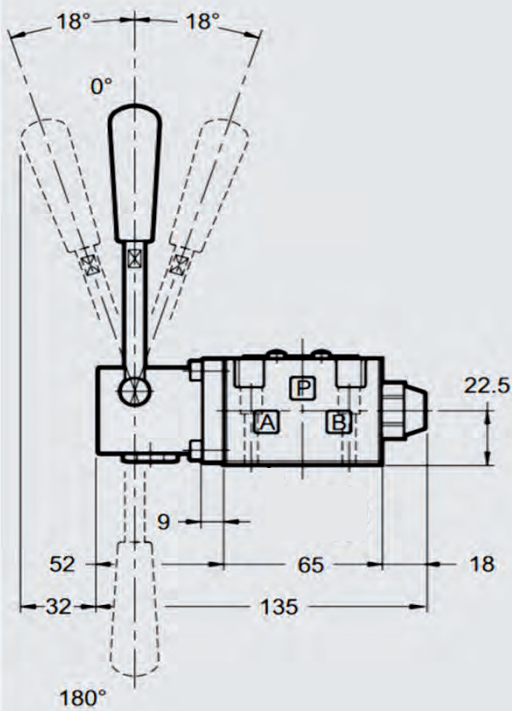
4/3-way
