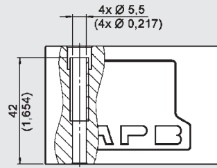
Clamping length
