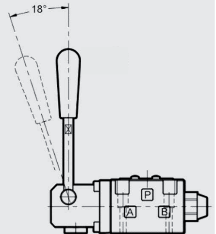
4/2-way
